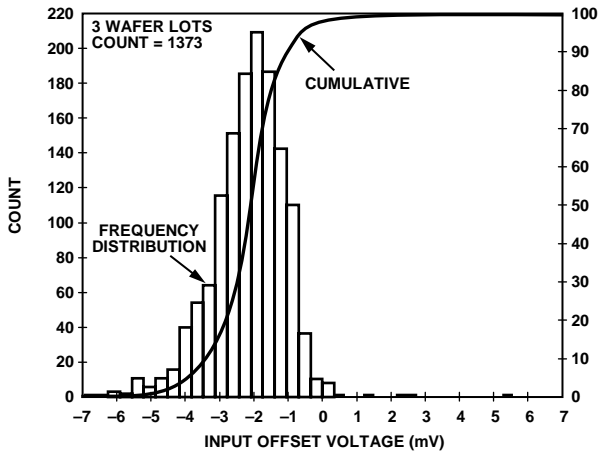
Figure 55. AD9631 Input Offset Voltage Distribution
