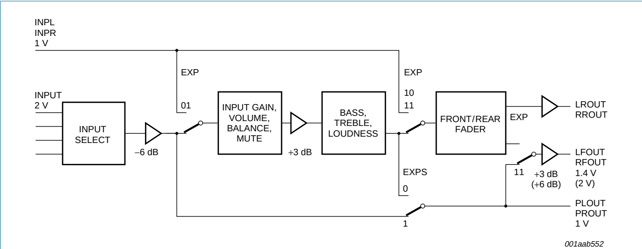
Fig 39. External processor connections
