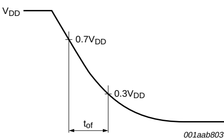
Fig 43. Definition of the fall time of the output signal
