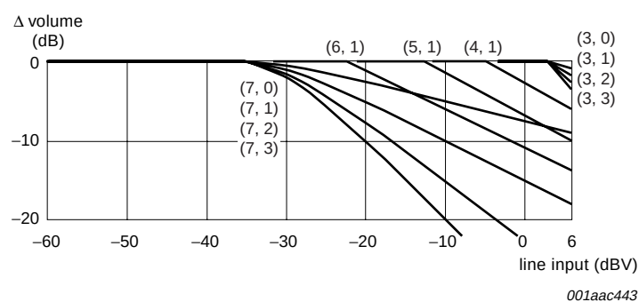
Fig 34. Dynamic compression volume control; non-standard characteristics
