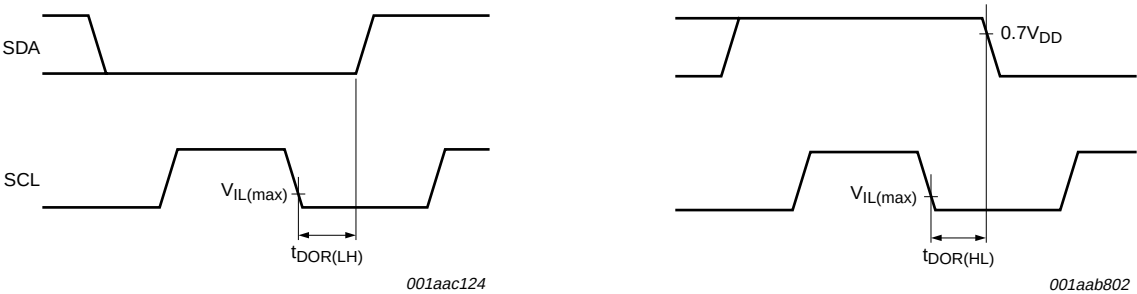
a. Data change from LOW to HIGH. b. Data change from HIGH to LOW.
