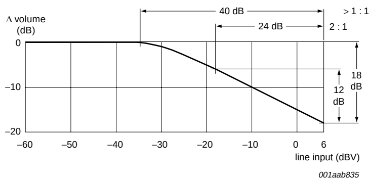
Fig 35. Dynamic compression volume control; typical setting
