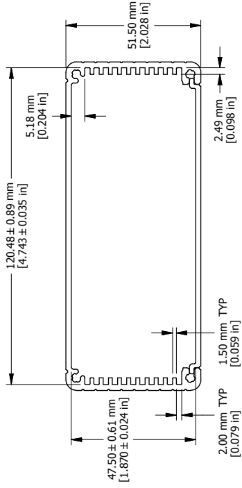
EXTRUSION
