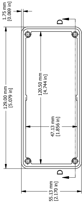
EXTRUSION DESIGNED FOR 120MM WIDE PC BOARD
