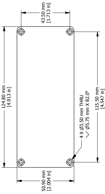
END PLATE
