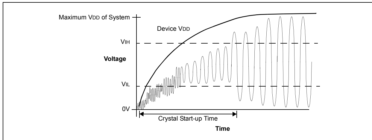
FIGURE 3-4: EXAMPLE OSCILLATOR/RESONATOR START-UP CHARACTERISTICS
