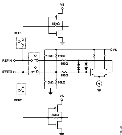
Figure 43. REF1N Equivalent Circuit for Non-XTAL Mode
