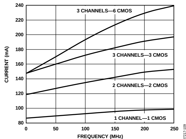
Figure 7. Total Current vs. Frequency, CLK-to-Output (PLL Off), CMOS Outputs with 10\text{ pF} Load
