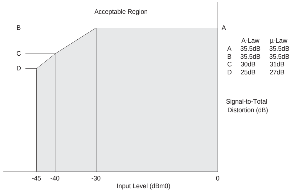
Figure 6. Total Distortion with Tone Input (Both Paths)
