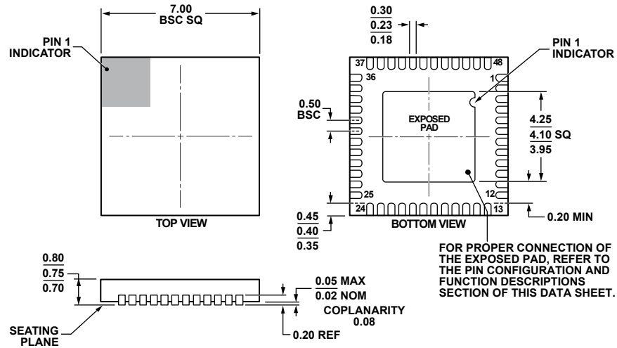
Figure 52. 48-Lead Lead Frame Chip Scale Package [LFCSP_WQ] 7 mm x 7 mm Body, Very Thin Quad (CP-48-5) Dimensions shown in millimeters
