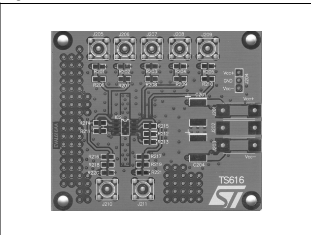
Figure 56. Evaluation board
