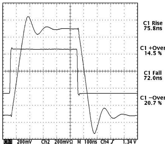
Figure 57. LMP7715 Response Gain = +2
