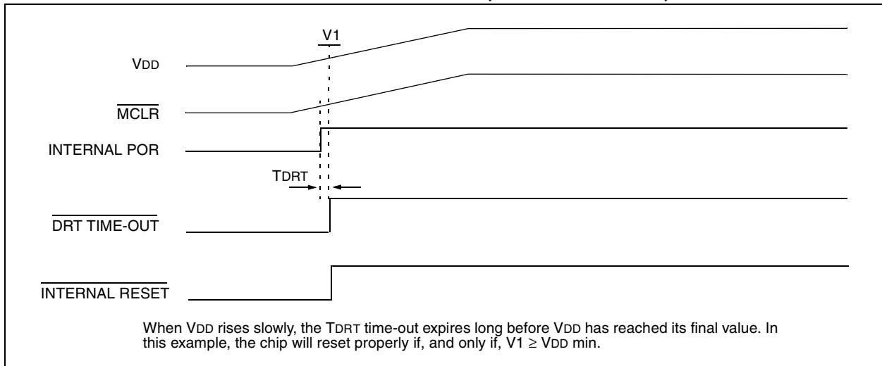
FIGURE 7-10: TIME-OUT SEQUENCE ON POWER-UP ( \overline{\text{MCLR}} TIED TO V_{DD} ): SLOW V_{DD} RISE TIME
