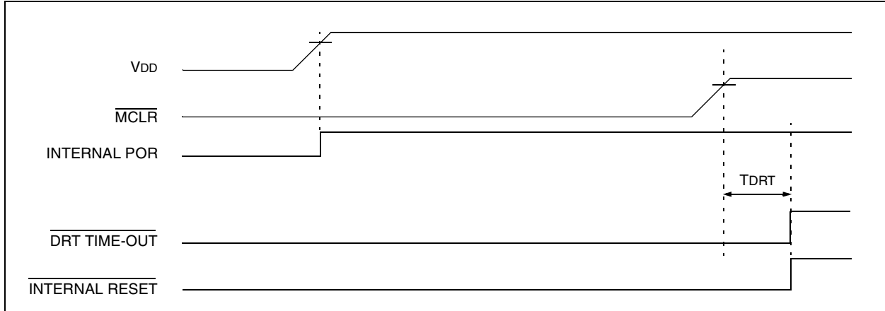
FIGURE 7-8: TIME-OUT SEQUENCE ON POWER-UP ( \overline{\text{MCLR}} NOT TIED TO V_{DD} )
