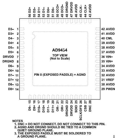
Figure 4. Pin Configuration—Single Data Rate Mode
