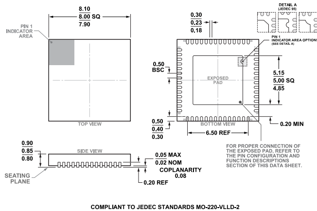
COMPLIANT TO JEDEC STANDARDS MO-220-VLLD-2 Figure 53. 56-Lead Lead Frame Chip Scale Package [LFCSP] 8 mm × 8 mm Body and 0.85 mm Package Height (CP-56-21) Dimensions shown in millimeters
