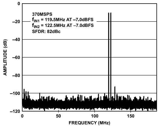
Figure 26. AD9434-370 64k Point, Two-Tone FFT; 370 MSPS, 119.5 MHz, 122.5 MHz
