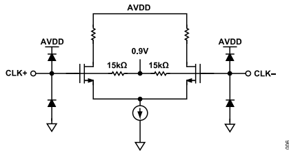
Figure 33. Clock Inputs
