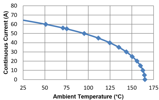
Figure 4: Maximum Continuous Current at a Given T_A
