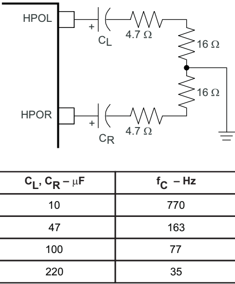
Figure 42. High-Pass Filter for Headphone Output
