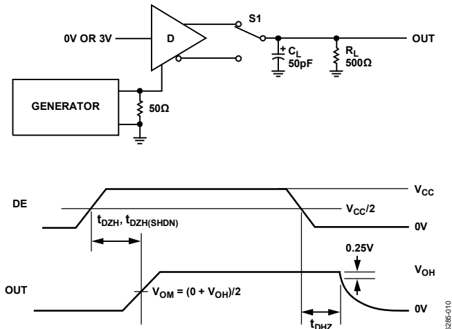
Figure 10. Driver Enable and Disable Times ( t_{DZH} , t_{DZH(SHDN)} , t_{DZL} , t_{DLZ} )
