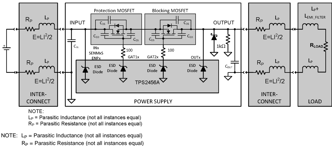
Figure 22. System Transient Model
