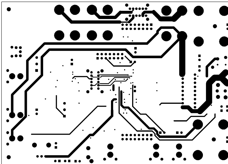
Figure 6-4. Mid Layer 2
