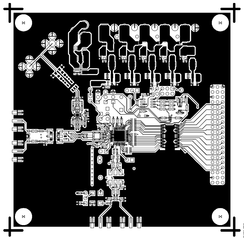
Figure 65. Evaluation Board Layout, Primary Side
