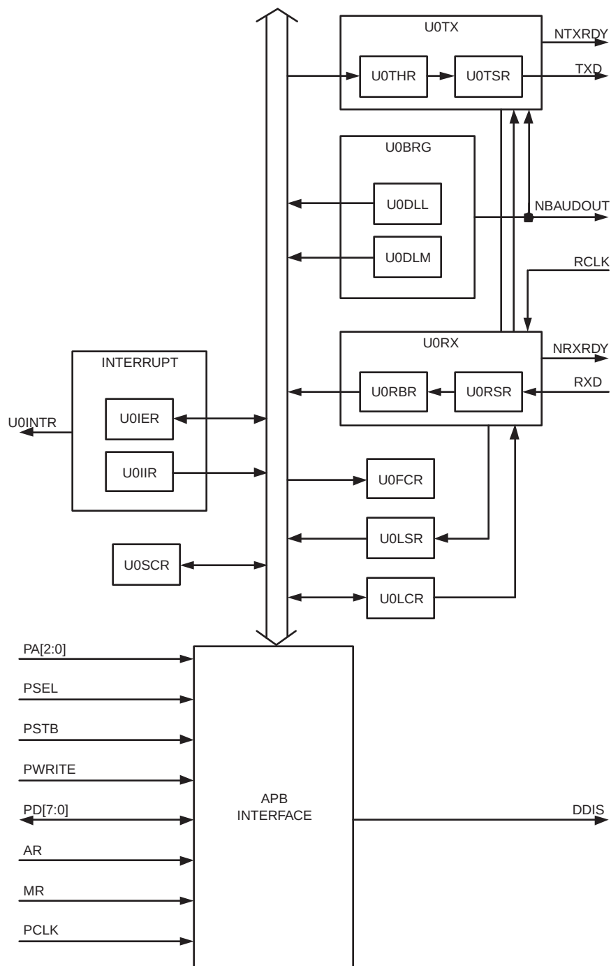
Fig 36. UART block diagram
