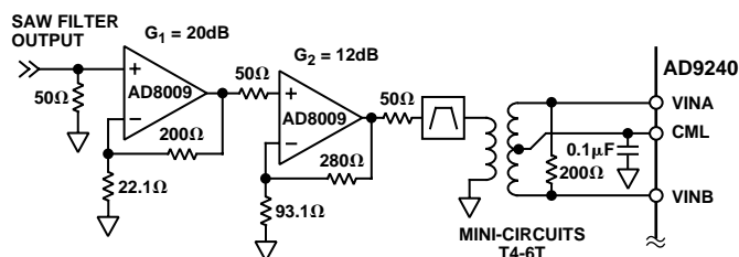
Figure 52. Simplified AD9240 IF Sampling Circuit
