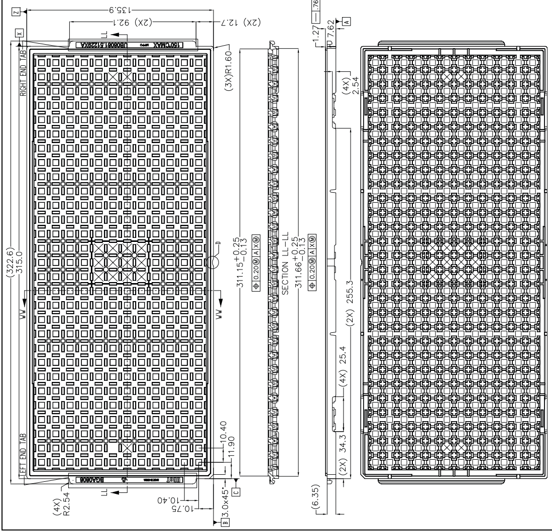
Figure 36. CYW20733 8 x 8 FBGA Package Tray (1 of 2)
