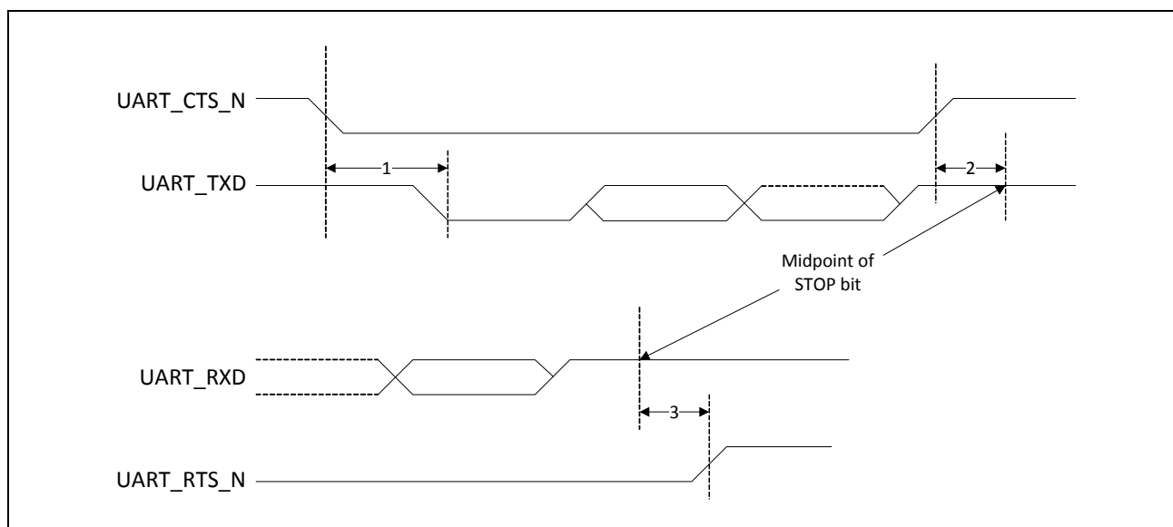
Figure 15. UART Timing
