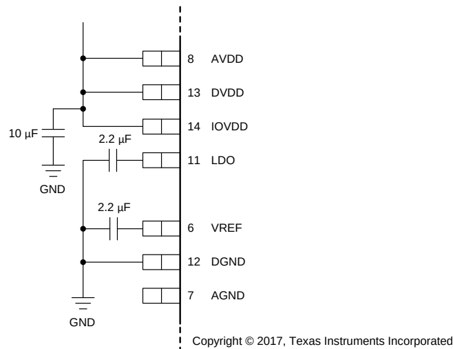
Figure 58. Single 3.3-V Supply
