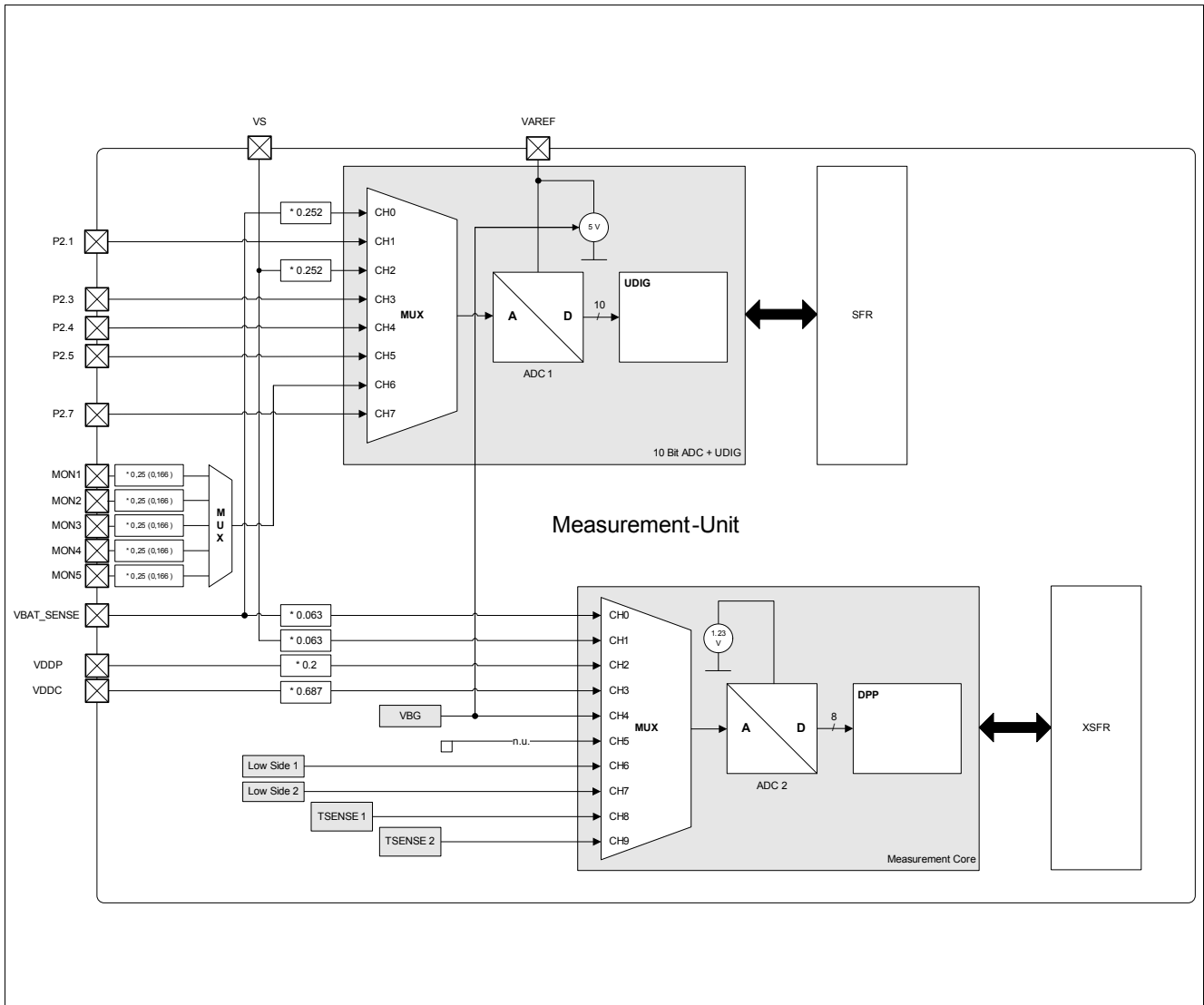
Figure 25 TLE9832 Measurement Unit-Overview
