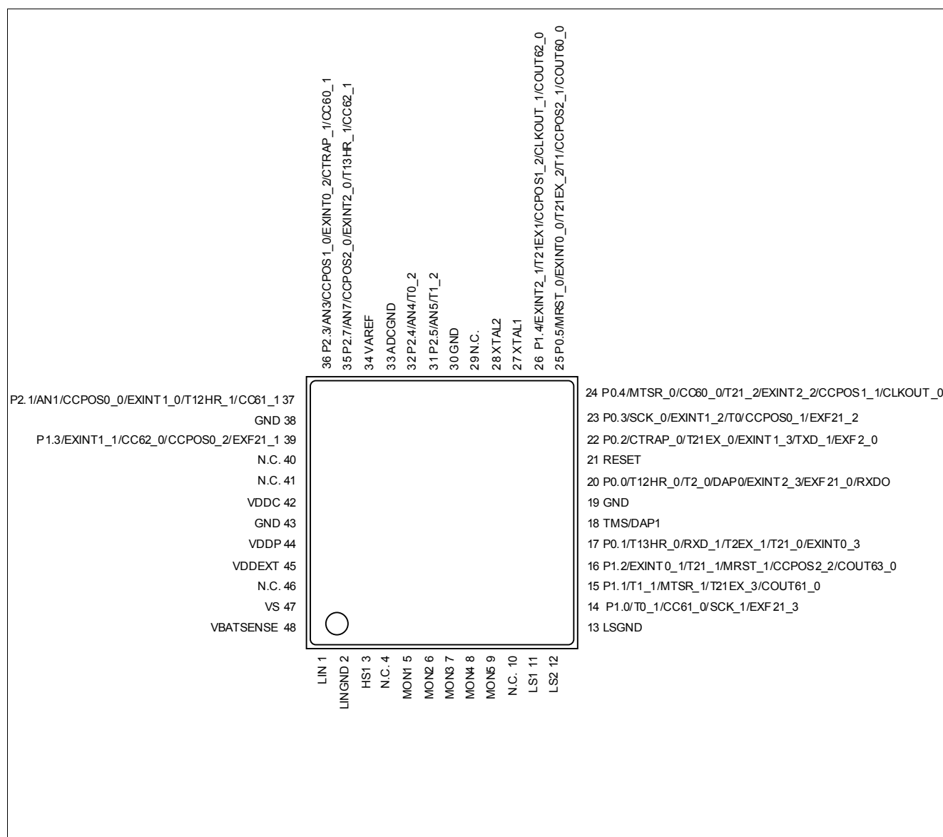
Figure 1 TLE9832 pin configuration, VQFN-48-22 and VQFN-48-29 package (top view)
