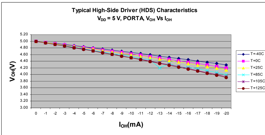
Figure 10. Typical High-Side Driver (Source) Characteristics High Drive ( PTxDSn = 1 ), V_{DD} = 5.0\text{ V} , V_{OH} vs. I_{OH}
