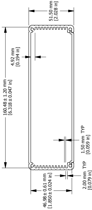
EXTRUSION
