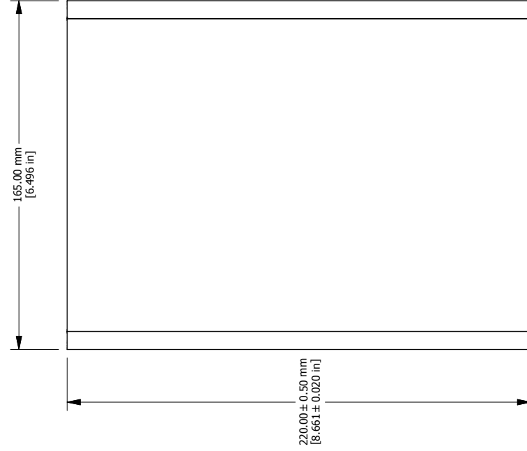
EXTRUSION DESIGNED FOR 160MM WIDE PC BOARD
