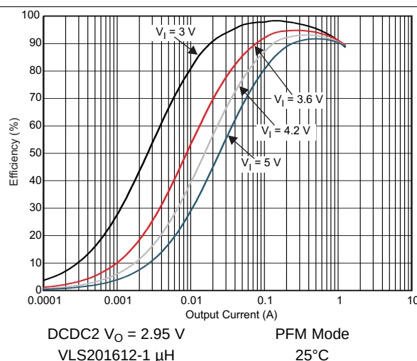
Figure 5-12. DCDC2 Efficiency vs Output Current / PWM Mode
