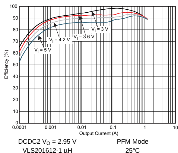
Figure 5-11. DCDC2 Efficiency vs Output Current / PFM Mode
