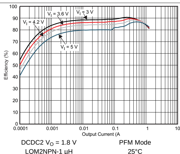
Figure 5-7. DCDC2 Efficiency vs Output Current / PFM Mode
