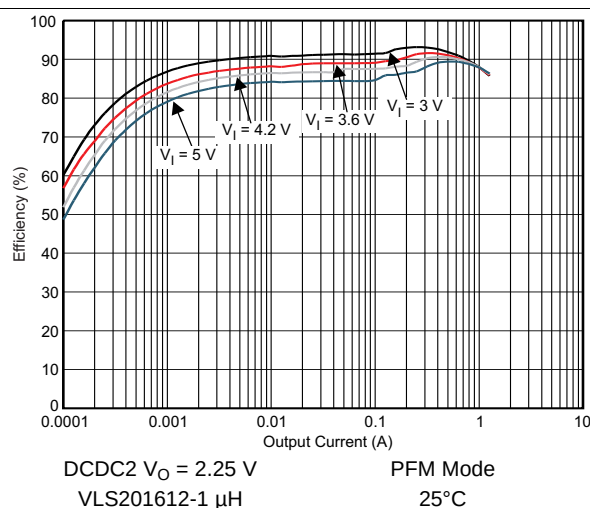
Figure 5-9. DCDC2 Efficiency vs Output Current / PFM Mode
