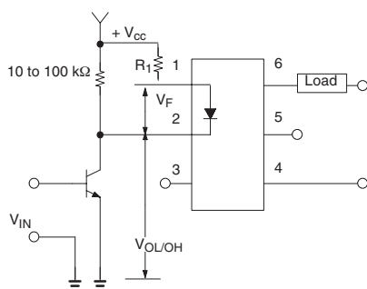
Transistor
