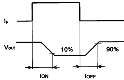
Timing Chart
