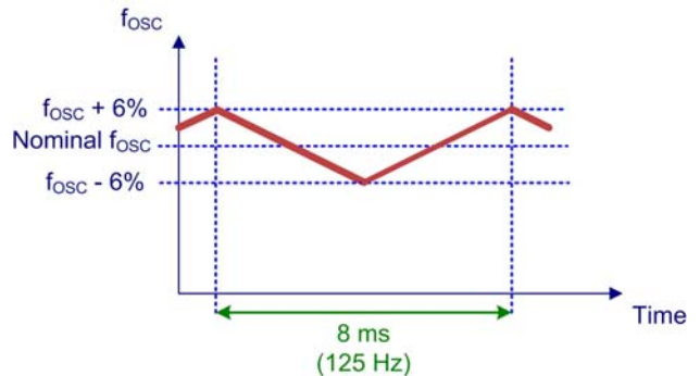
Figure 55. Frequency Modulation of the Maximum Switching Frequency
