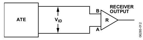
Figure 12. Receiver Propagation Delay Test Circuit
