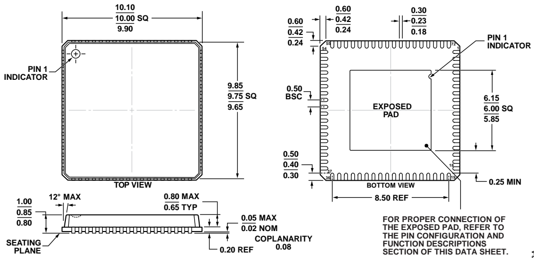
Figure 65. 72-Lead Lead Frame Chip Scale Package [LFCSVP_VQ] 10 mm × 10 mm Body, Very Thin Quad (CP-72-7) Dimensions shown in millimeters
