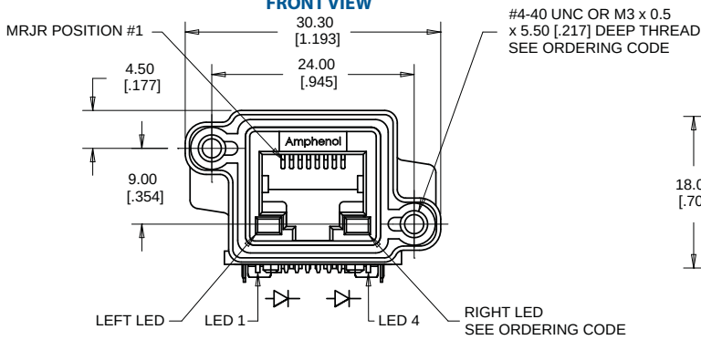
FRONT VIEW
