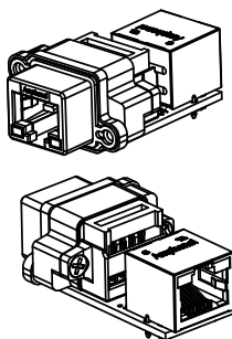
ISOMETRIC VIEWS
