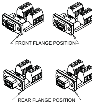
ISOMETRIC VIEWS
