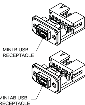
ISOMETRIC VIEWS
