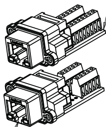
4, 6, OR 8 (WITHOUT LED'S) CONTACT RECEPTACLE
