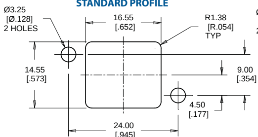
STANDARD PROFILE
