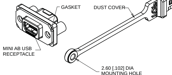
ISOMETRIC VIEWS
