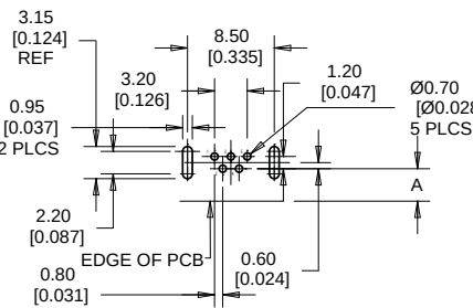
LOW PROFILE
