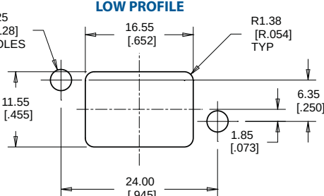
LOW PROFILE
