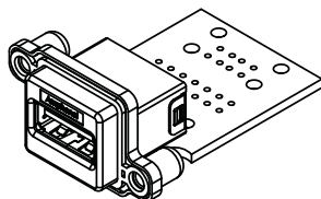
ISOMETRIC VIEW
