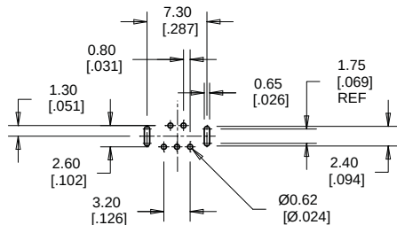
STANDARD PROFILE
