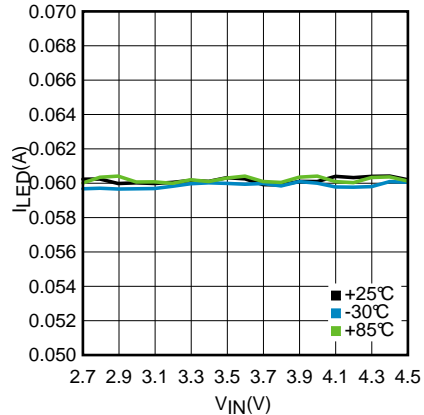
Figure 8. 60mA Torch LED Current vs Input Voltage
