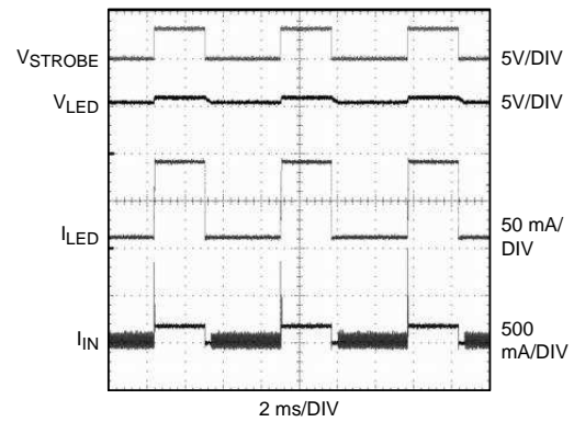
Figure 34. Assist PWM
