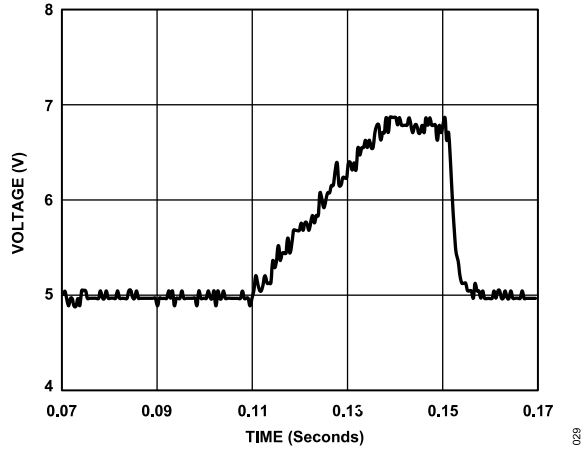
Figure 37. V_{EXT\_CAP} Waveform While Writing Fuse
