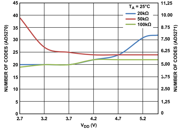
Figure 34. Maximum Code Loss > 1% R-Tolerance Error vs. Voltage
