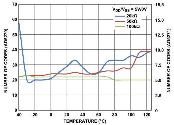
Figure 35. Maximum Code Loss > 1% R-Tolerance Error vs. Temperature
