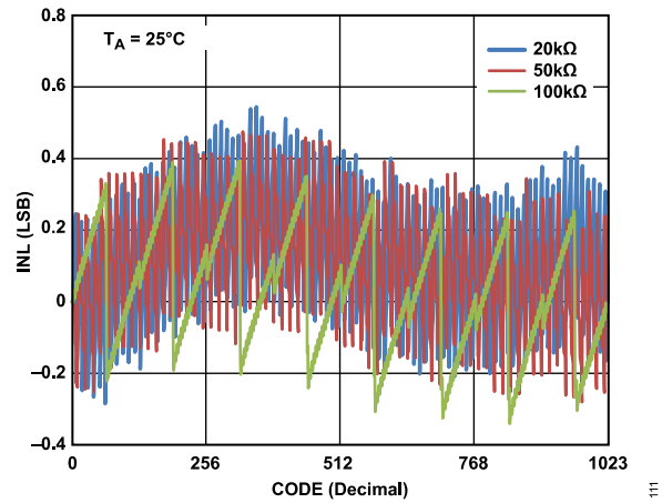
Figure 8. R-INL in R-Perf Mode vs. Code vs. Nominal Resistance (AD5270)
