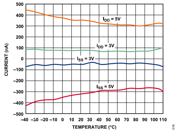
Figure 23. Supply Current ( I_{DD} , I_{SS} ) vs. Temperature
