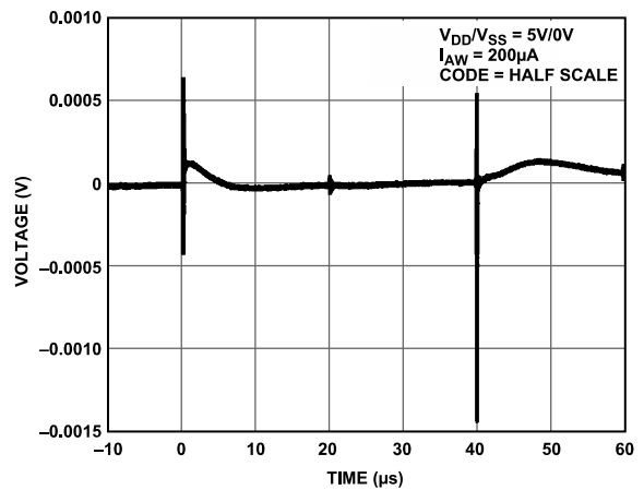
Figure 36. Digital Feedthrough
