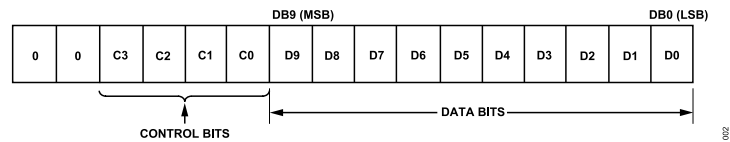
Figure 2. Shift Register Content
