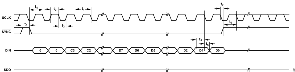
Figure 3. Write Timing Diagram (CPOL = 0, CPHA = 1)
