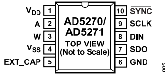
Figure 5. MSOP Pin Configuration
