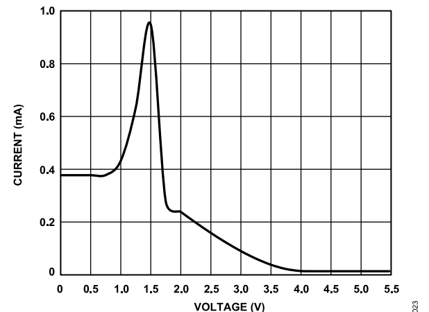
Figure 24. Supply Current I_{DD} vs. Digital Input Voltage
