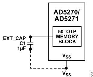
Figure 46. EXT_CAP Hardware Setup
