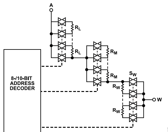
Figure 45. Simplified RDAC Circuit
