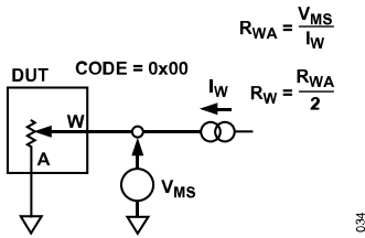
Figure 40. Wiper Resistance
