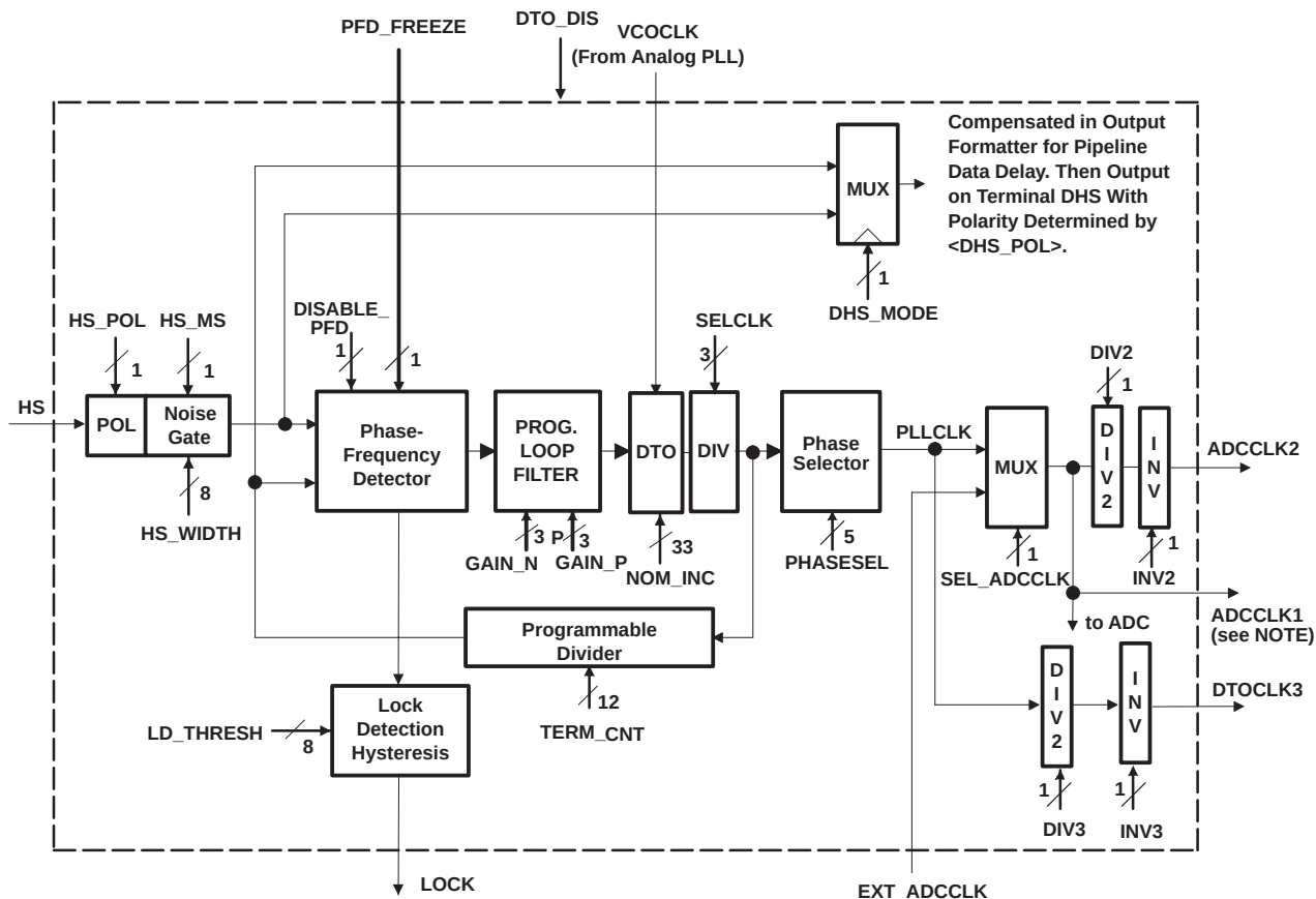
Figure 2-6. Digital PLL
