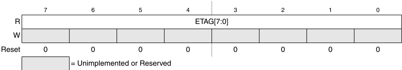
Figure 28-19. EEE Tag Counter Low Register (ETAGLO)
