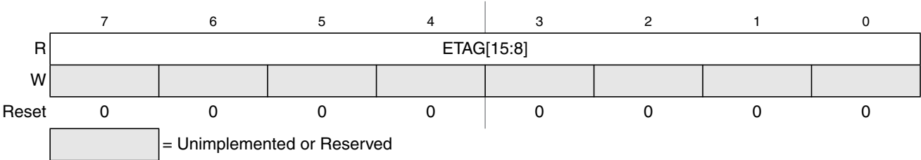
Figure 28-18. EEE Tag Counter High Register (ETAGHI)
