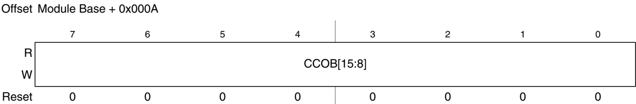
Figure 27-16. Flash Common Command Object High Register (FCCOBHI)
