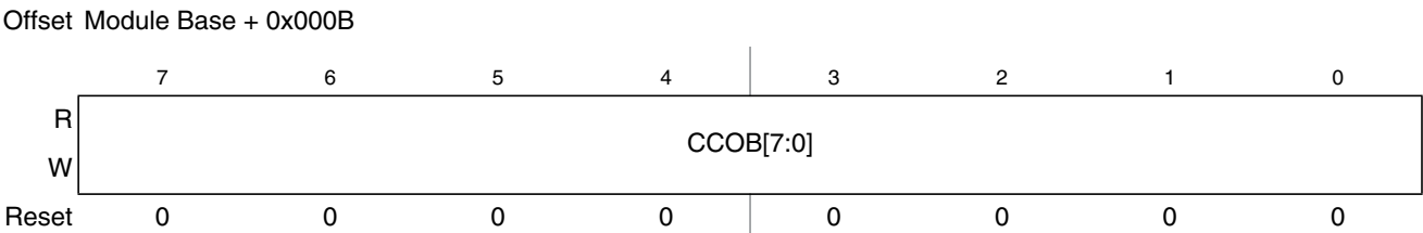
Figure 27-17. Flash Common Command Object Low Register (FCCOBLO)
