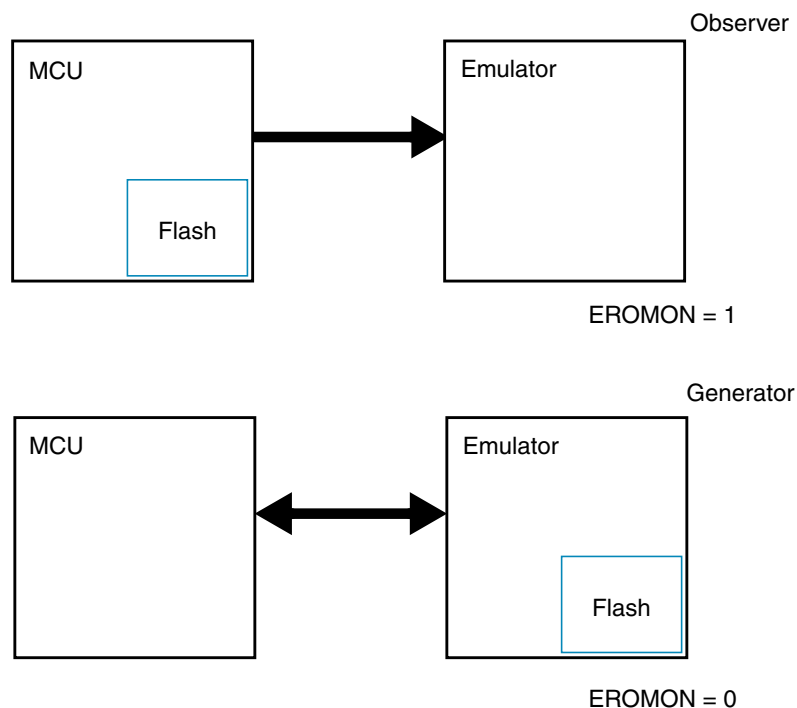
Figure 3-25. ROM in Emulation Single-Chip Mode
