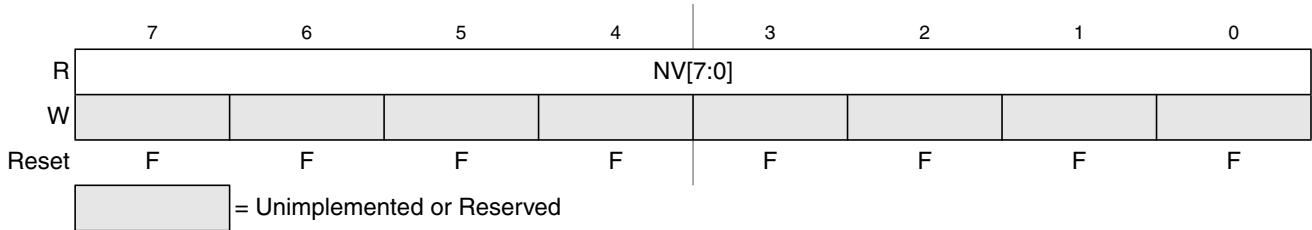
Figure 26-22. Flash Option Register (FOPT)
