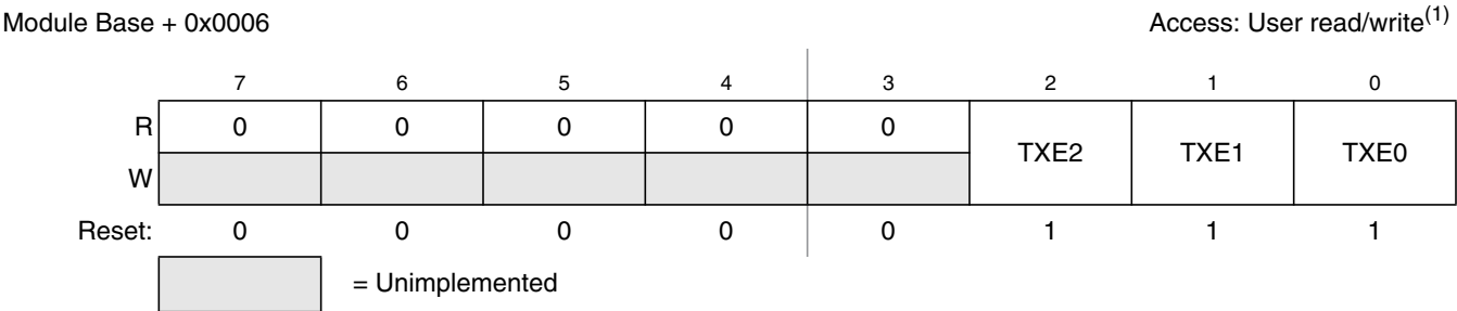
Figure 16-10. MSCAN Transmitter Flag Register (CANTFLG)
