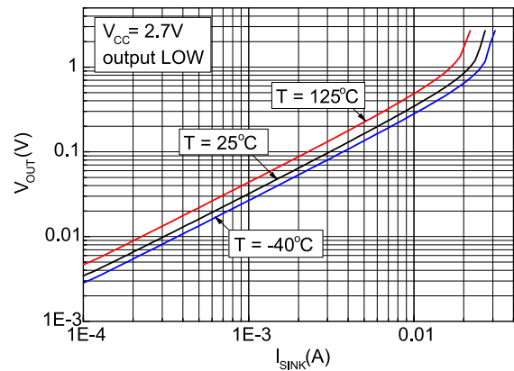
Figure 4: Output voltage vs. sinking current, output low, V_{CC} = 2.7\text{V}
