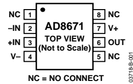
Figure 1. 8-Lead SOIC_N (R-8) and 8-Lead MSOP (RM-8)
