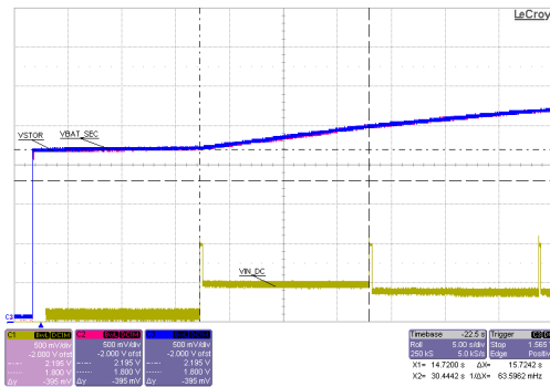
Sourcemeter with V_{SOURCE} = 1.0\text{ V} and compliance of 8.5\text{ mA} subsequently applied to V_{IN\_DC} V_{BAT} = 0.1\text{ F} capacitor charged to 2.2\text{ V} Resistance on V_{STOR} = 100\text{ k}\Omega
