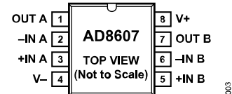
Figure 3. 8-Lead SOIC (R Suffix)
