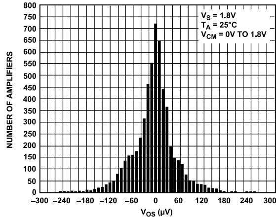
Figure 28. V_{OS} Distribution
