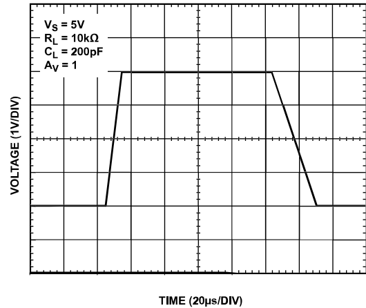
Figure 23. Large Signal Transient
