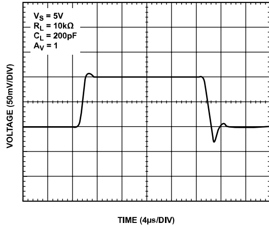
Figure 22. Small Signal Transient
