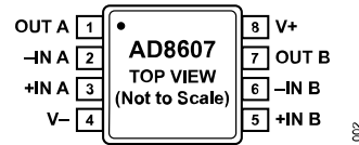
Figure 2. 8-Lead MSOP (RM Suffix)
