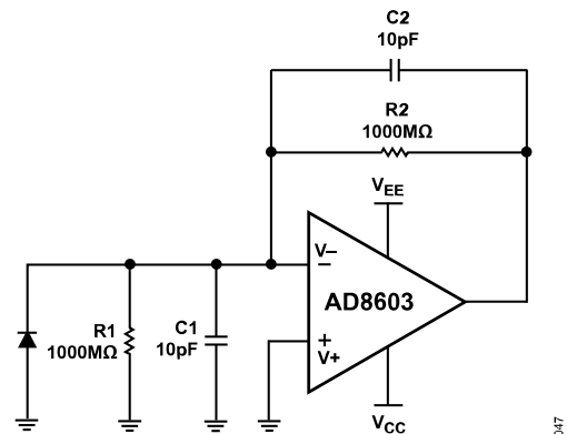
Figure 47. Photodiode Circuit
