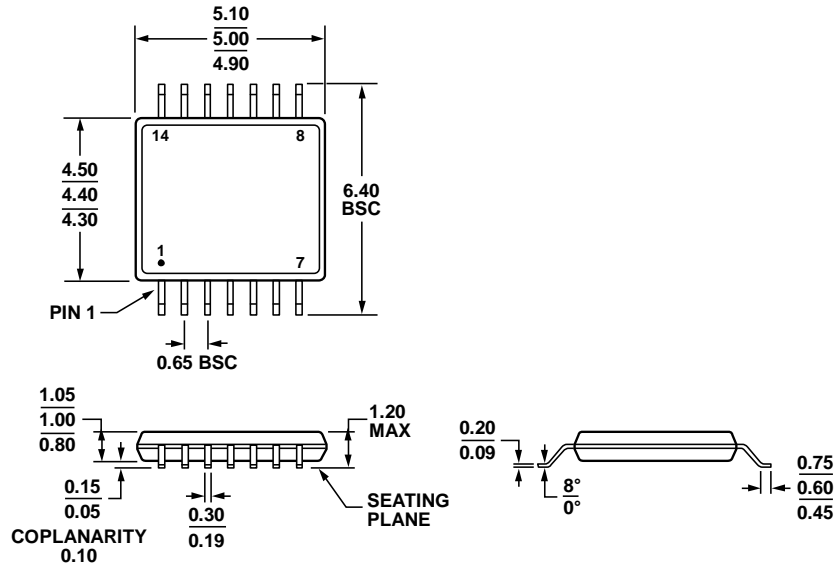
Figure 63. 14-Lead Thin Shrink Small Outline Package [TSOP] (RU-14)
