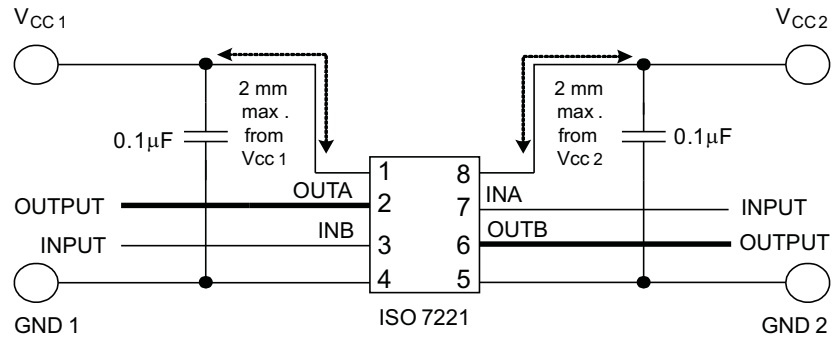
Figure 14. Typical ISO7221 Application Circuit
