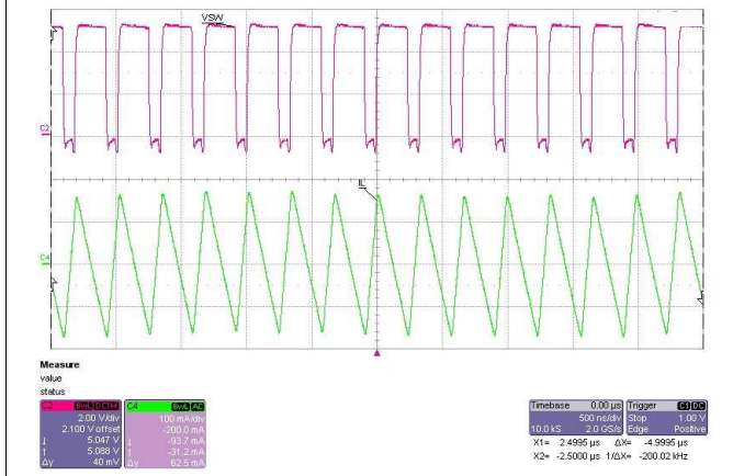
Figure 30. 1.0 µH CCM Operation
