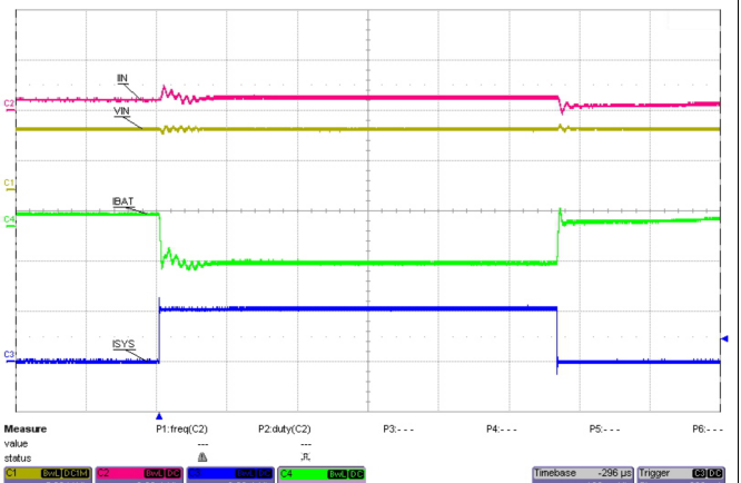
Figure 31. 2A Load Step Transient
