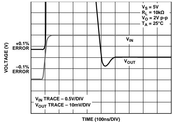
Figure 51. Settling Time
