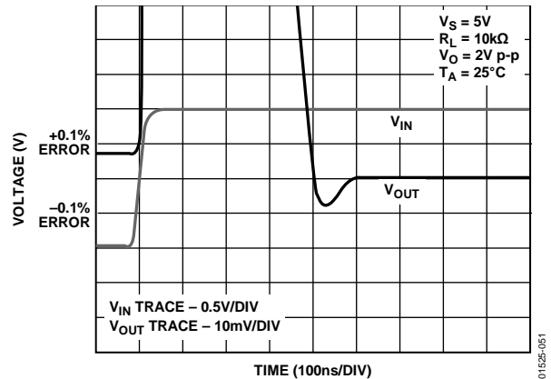
Figure 51. Settling Time
