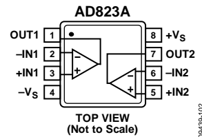
Figure 2. 8-Lead MSOP
