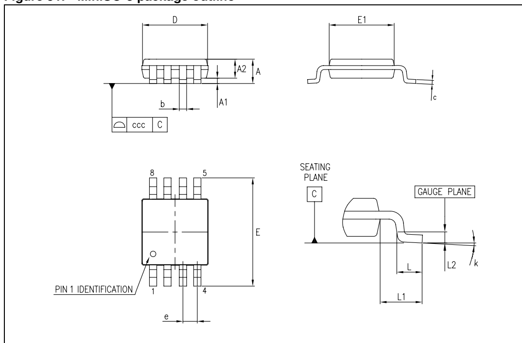
Figure 51. MiniSO-8 package outline
