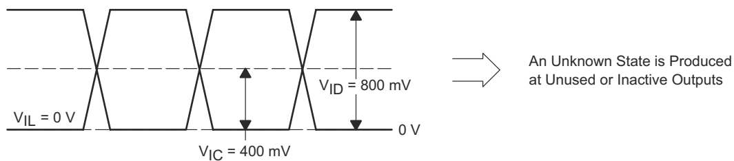
Figure 8-6. Waveform 4
