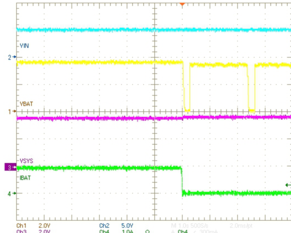
Figure 31. Battery Removal
