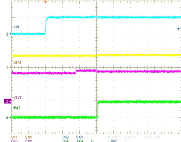
Figure 32. Default Start-up - bq24260 (D+/D- Shorted)
