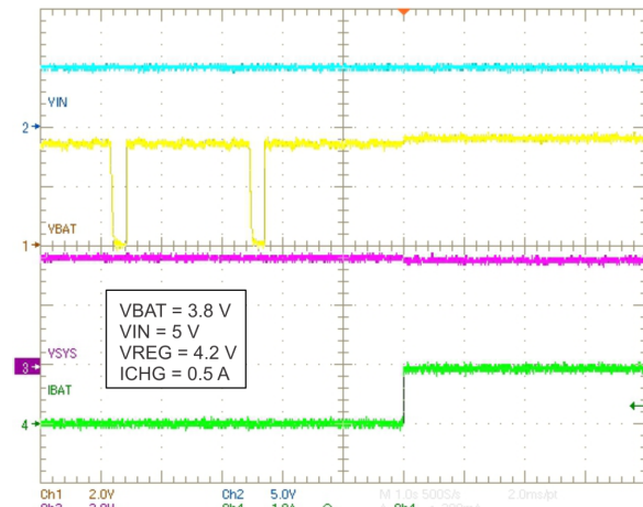
Figure 30. Battery Detection
