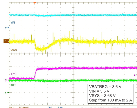
Figure 34. VSYS Transient Without Supplement Mode
