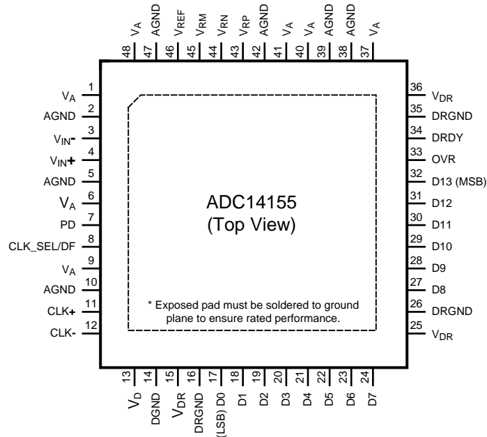
Figure 1. 48-Lead WQFN Package Package Number RHS0048A
