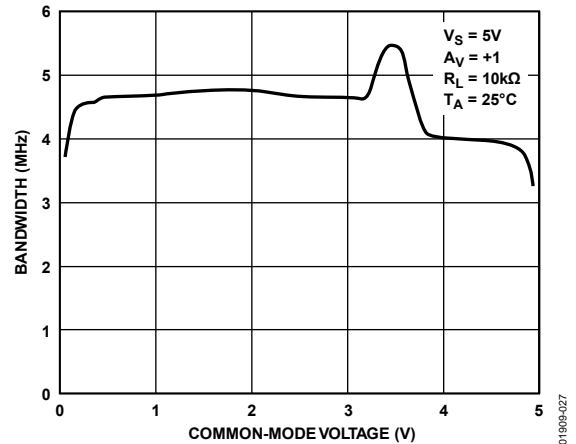
Figure 27. Frequency vs. Common-Mode Voltage ( V_S = 5V )
